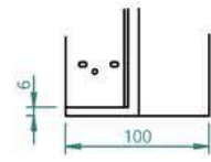
Fig. 3 Threshold Detail D (1:5)
