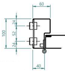
Fig. 4 Detail B (1:5)
