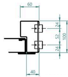
Fig. 5 Detail C (1:5)
